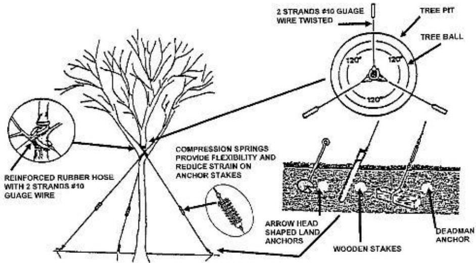
Figure 15. Support and Anchorage of Large Transplanted Trees
