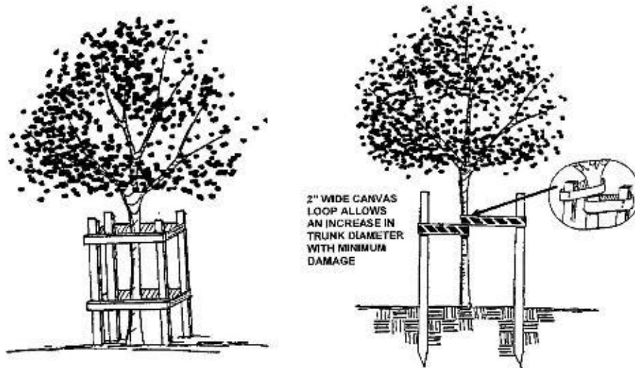
Figure 15. Support and Anchorage of Large Transplanted Trees
